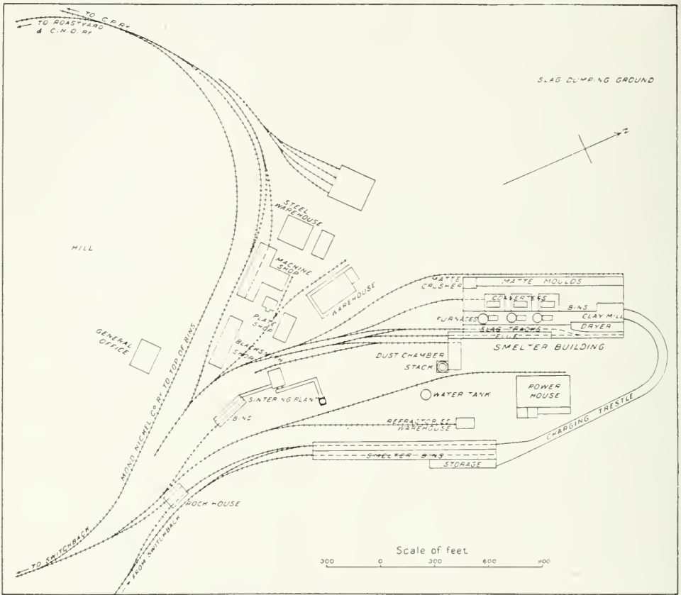
Fig. 79—Plan of Smelter and Adjacent Buildings, Mond Nickel Company, Coniston, Ontario.
